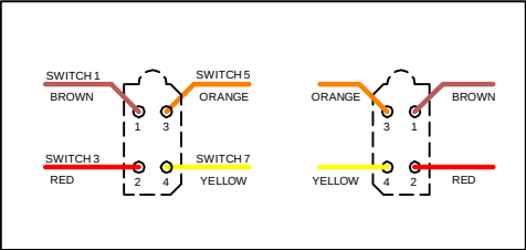
4 PIN MATE 'N' LOCK MOLEX
